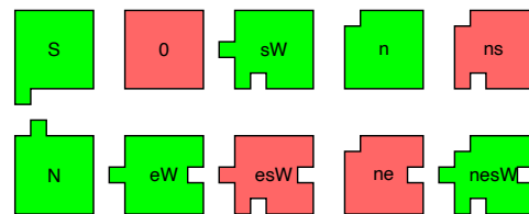
Figure 3: Tiles for binary subtraction:
